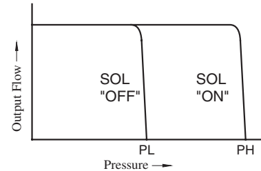
Performance Characteristics
