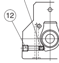
Section Y-Y
